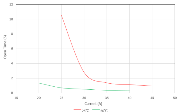
Open Time vs. Current Curves – @ 25°C & 60°C
