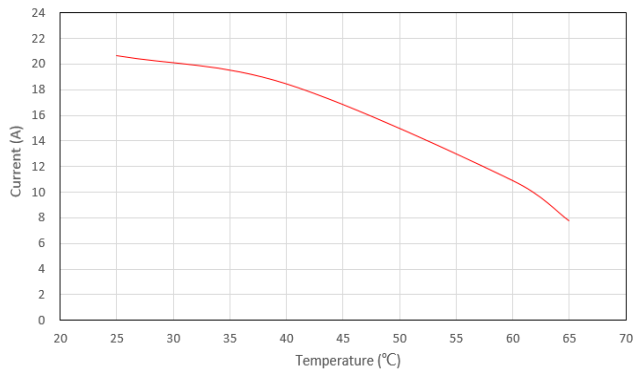
Current vs. Temperature Curve*
