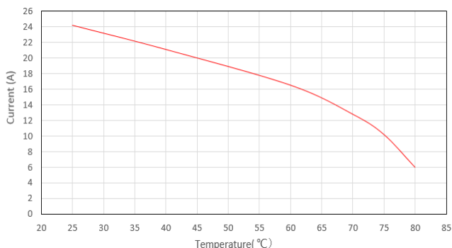
Current vs. Temperature Curve*
