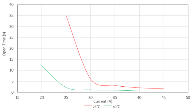
Open Time vs. Current Curves – @ 25°C & 60°C
