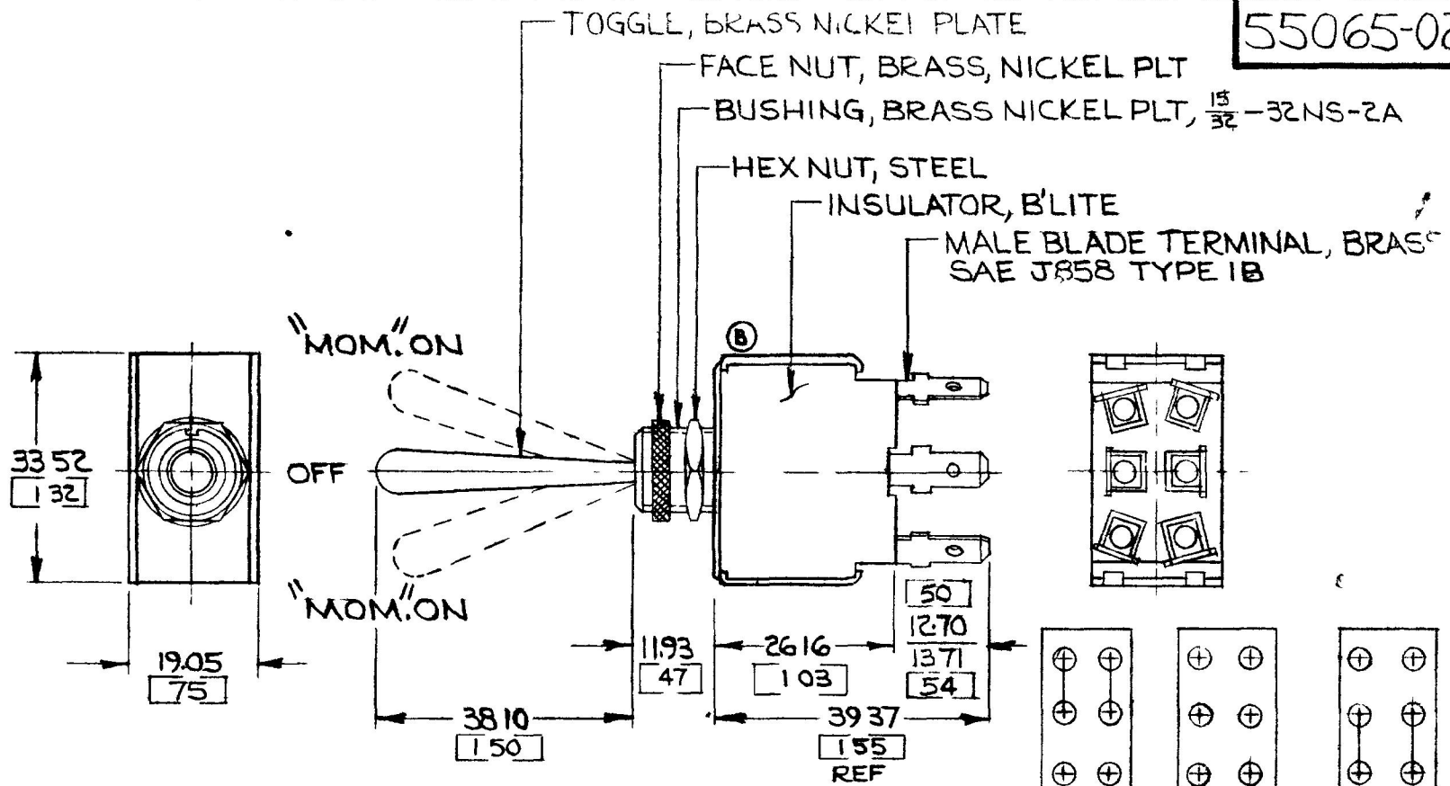
MOM. ON OFF MOM. ON CIRCUIT DIAGRAM
