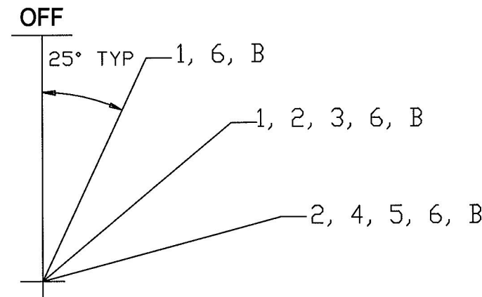
SWITCH OPERATION
