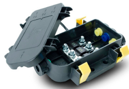
04980933.X MDB Series 3 Way Loaded Sealed MIDI® Fuse Holder
