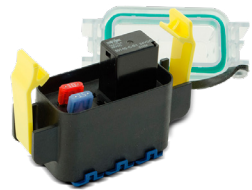
PDM33003ZXM HWB12 Series 12 Way Power Distribution Module
