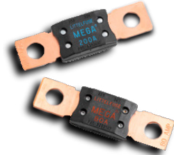
MEGA® FUSES 80A - 500A
