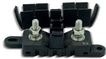
02981028HXFC-SS MEGA® Flex 32V 500A Bolt-Down Fuse Holder
