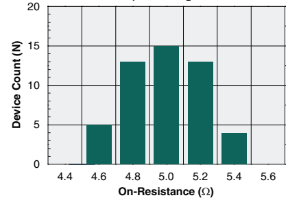
Typical On-Resistance Distribution (N=50, I_F=2\text{mA} , I_L=150\text{mA} )
