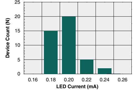
Typical I_F for Switch Dropout (N=50, I_L=400\text{mA} )
