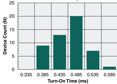
Typical Turn-On Time Distribution (N=50, I_F=5mA , I_L=100mA )
