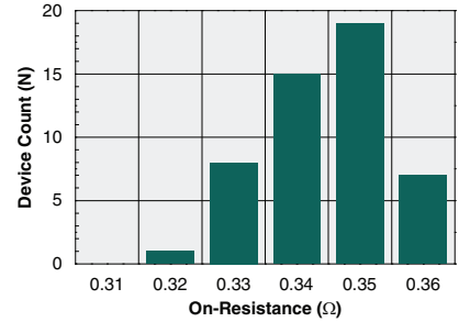
Typical On-Resistance Distribution (N=50, I_F=2mA , I_L=0.75A )
