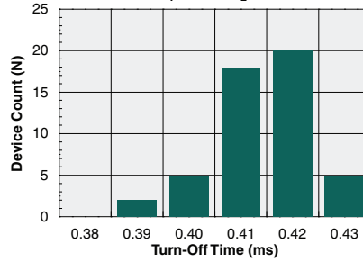
Typical Turn-Off Time Distribution (N=50, I_F=5mA , I_L=100mA )
