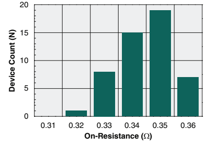
Typical On-Resistance Distribution (N=50, I_F=2mA , I_L=0.75A )
