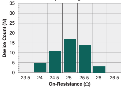
Typical On-Resistance Distribution (N=50, I F =2mA, I L =120mA)
