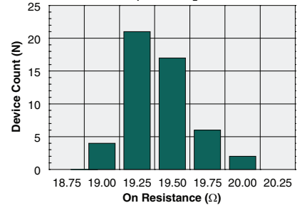
Typical On-Resistance Distribution (N=50, I_F=5\text{mA} , I_L=120\text{mA} )
