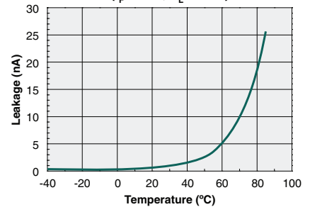
Typical Leakage vs. Temperature Measured Across Pins 3&4 ( I_F=0mA, V_L=350V )
