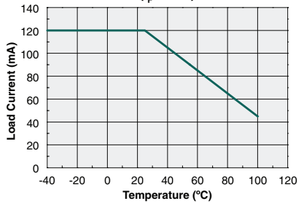
Maximum Load Current vs. Temperature ( I_F=4mA )
