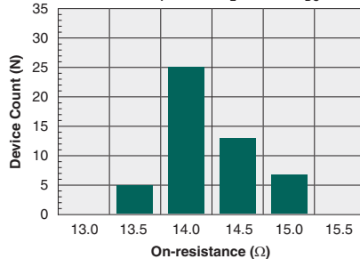
Typical On-Resistance Distribution (N=50, I F =2mA, I L =140mA DC )
