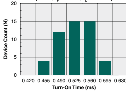
Typical Turn-On Time (N=50, I F =10mA, I L =140mA)
