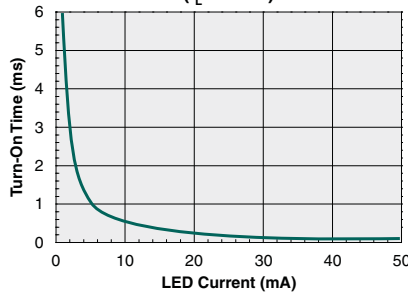
Typical Turn-On Time vs. LED Forward Current (I L =70mA)
