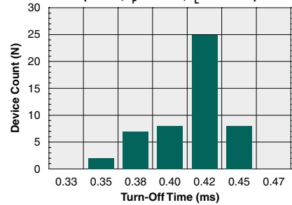
Typical Turn-Off Time (N=50, I F =10mA, I L =140mA)
