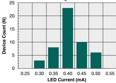
Typical I F for Switch Operation (N=50, I L =140mA)
