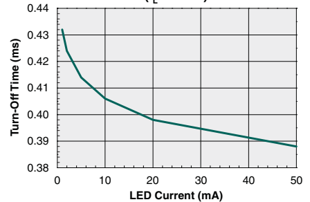
Typical Turn-Off Time vs. LED Forward Current (I L =70mA)
