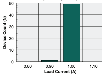
Typical Current Limit Distribution (N=50, I F =5mA)
