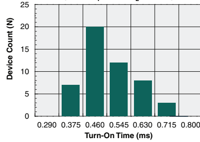
Typical Turn-On Time (N=50, I_F=5mA , I_L=75mA )
