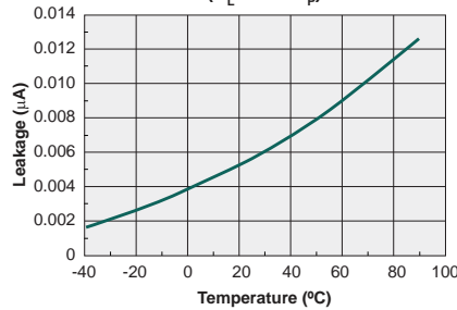
Typical Leakage vs. Temperature Measured Across Pins 1&2 ( V_L = 1000V_r )
