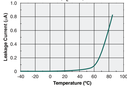
Leakage Current vs. Temperature Across Pins 5&6, 7&8 ( V_L=60V )
