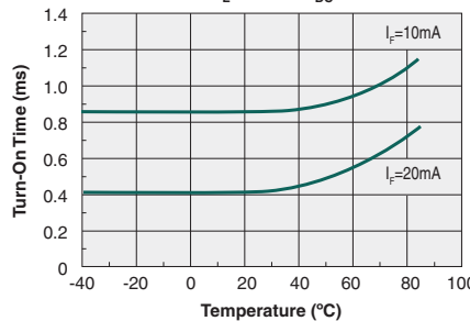
Typical Turn-On Time vs. Temperature ( I_L=100mA_{DC} )
