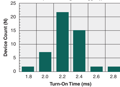
Typical Turn-On Time (N=50, I_F=10mA , I_L=5mA_{DC} , T_A=25^\circ C )
