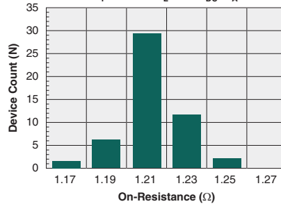
Typical On-Resistance Distribution (N=50, I_F=10mA , I_L=0.7A_{DC} , T_A=25^\circ C )
