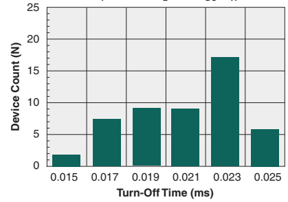
Typical Turn-Off Time (N=50, I_F=10mA , I_L=5mA_{DC} , T_A=25^\circ C )
