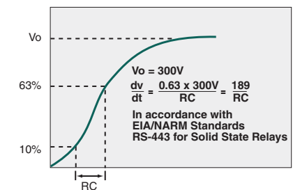
dV/dt Method
