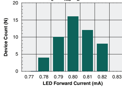
Typical I_F for Switch Operation ( I_L=1\text{A}_{\text{rms}} , T_A=25^\circ\text{C} )
