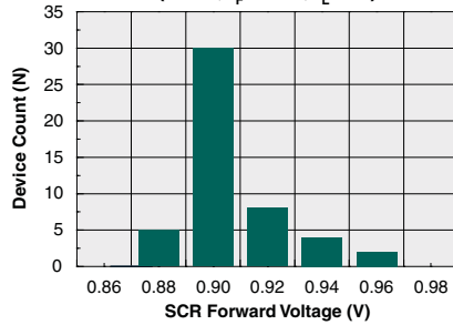
Typical SCR Forward Voltage Distribution (N=50, I_F=5\text{mA} , I_L=2\text{A} )
