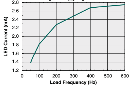
LED Current to Operate vs. Load Frequency ( V_L=140V_{rms} , R_L=400\Omega )
