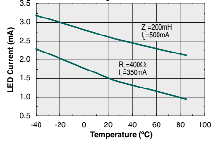
LED Current to Operate (f o =60Hz)
