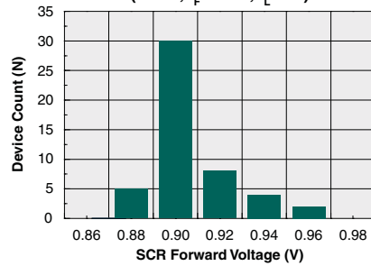
Typical SCR Forward Voltage Distribution (N=50, I F =5mA, I L =2A)
