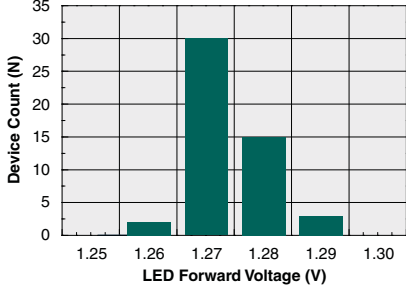
LED Forward Voltage Distribution (N=50, I F =5mA)
