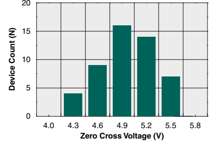
Zero Cross Voltage Distribution (N=50, I F =5mA)
