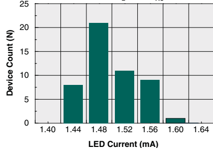
LED Current to Operate Distribution (60Hz Resistive Load) (N=50, V L =120V AC )
