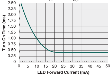
Typical Turn-On Time vs. LED Forward Current ( I_L = 100\text{mA}_{\text{DC}} )
