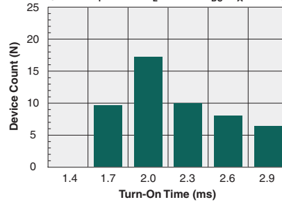
Typical Turn-On Time (N=50, I_F=5mA , I_L=120mA_{DC} , T_A=25^\circ C )
