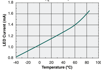
Typical I F for Switch Operation vs. Temperature (I L =300mA)
