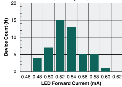
Typical I F for Switch Operation (N=50, I L =1A)
