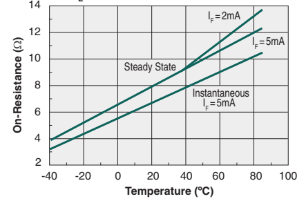
Typical On-Resistance vs. Ambient Temperature ( I_L=\text{Max Rated @ Temperature} )
