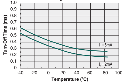
Typical Turn-Off Time vs. Ambient Temperature ( I_L=50\text{mA} )
