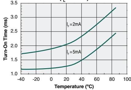
Typical Turn-On Time vs. Ambient Temperature ( I_L=50\text{mA} )
