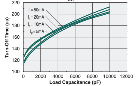
Turn-Off Time vs. Load Capacitance ( V_{OUT}=5\text{V} )
