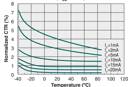
Typical Normalized CTR vs. Temperature ( V_{CE}=0.5\text{V} )
