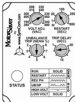
Figure 3: Adjustment Knobs
