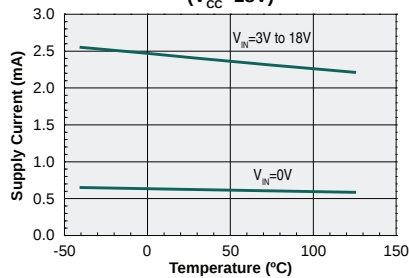
Quiescent Supply Current vs. Temperature ( V_{CC}=18V )
