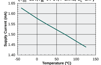
Dynamic Supply Current vs. Temperature Both Outputs Active ( V_{CC}=18V, V_{IN}=0V-5V, f=1kHz, C_L=1nF )
