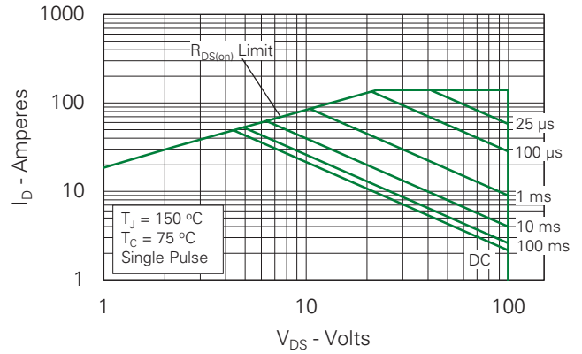
Fig. 14. Forward-Bias Safe Operating Area @ T_C = 75^\circ\text{C}
