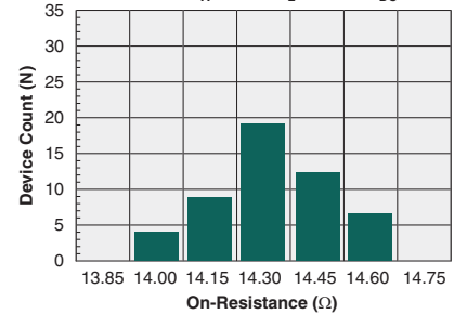
Typical On-Resistance Distribution (N=50, T_A=25^\circ C , I_L=120mA_{DC} )
