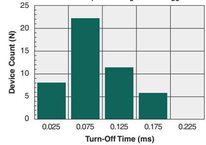
Typical Turn-Off Time (N=50, I_F=5mA , I_L=120mA_{DC} )
