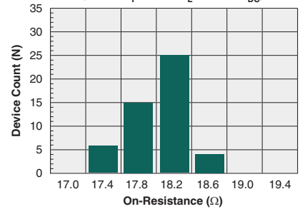
Typical On-Resistance Distribution (N=50, I_F=5mA , I_L=120mA_{DC} )
