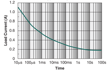
Form-B Energy Rating Curve
