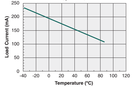
Form-B Maximum Load Current vs. Temperature ( I_F=0\text{mA} )
