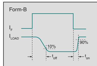
Switching Characteristics of Normally Closed Devices
