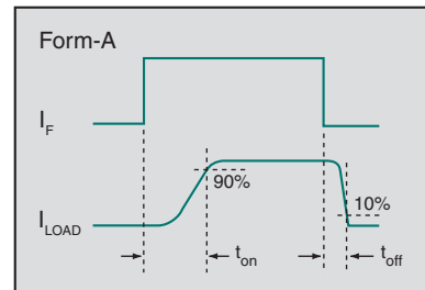
Switching Characteristics of Normally Open Devices
