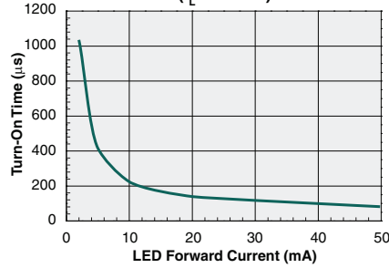
Form-A Typical Turn-On Time vs. LED Forward Current ( I_L=100mA )
