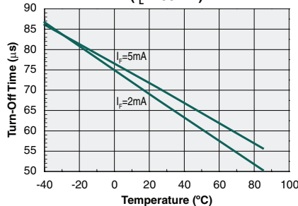
Form-A Typical Turn-Off Time vs. Temperature ( I_L=100mA )
