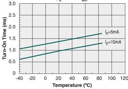
Typical Turn-On Time vs. Temperature ( I_L=80mA_{DC} )
