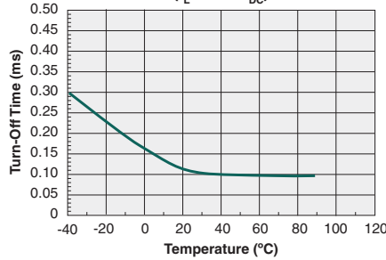
Typical Turn-Off Time vs. Temperature ( I_L=80mA_{DC} )
