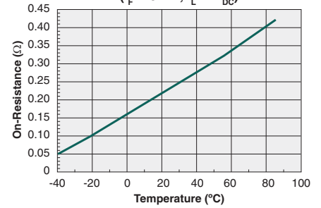
Typical On-Resistance vs. Temperature ( I_F=10mA, I_L=1A_{DC} )
