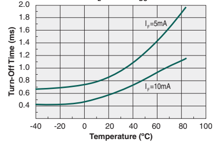
Typical Turn-Off Time vs. Temperature ( I_L=120mA_{DC} )
