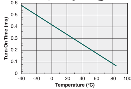
Typical Turn-On Time vs. Temperature ( I_F=5mA, I_L=120mA_{DC} )
