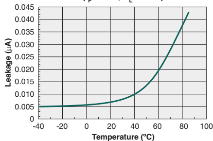
Typical Leakage vs. Temperature Measured Across Pins 4&6 ( I_F=5mA, V_L=350V )
