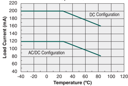
Maximum Load Current vs. Temperature ( I_F=0mA )
