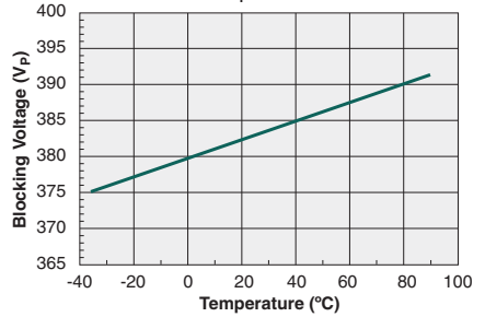
Typical Blocking Voltage vs. Temperature ( I_F=5mA )
