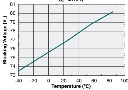
Typical Blocking Voltage vs. Temperature ( I_F=2mA )
