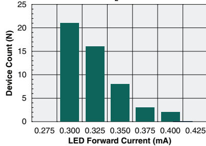
Typical LED Current to Operate (N=50, I_L=100\text{mA} )
