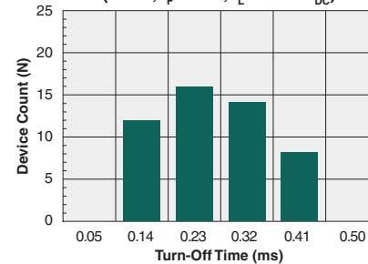
Form-A Typical Turn-Off Time (N=50, I_F=8\text{mA} , I_L=120\text{mA}_{DC} )
