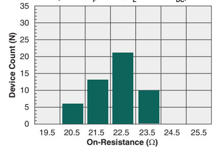
Form-A Typical On-Resistance Distribution (N=50, I_F=8\text{mA} , I_L=120\text{mA}_{DC} )
