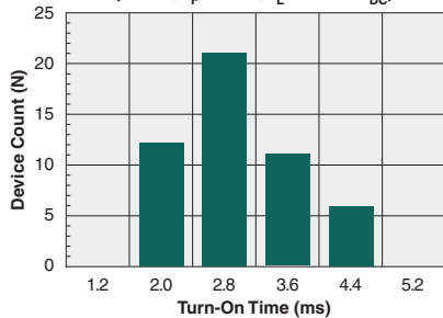
Form-A Typical Turn-On Time (N=50, I_F=8\text{mA} , I_L=120\text{mA}_{DC} )
