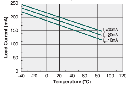
Form-A Maximum Load Current vs. Temperature
