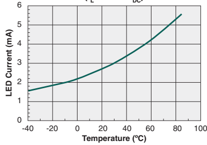
Form-A Typical I_F for Switch Dropout vs. Temperature ( I_L=170\text{mA}_{DC} )
