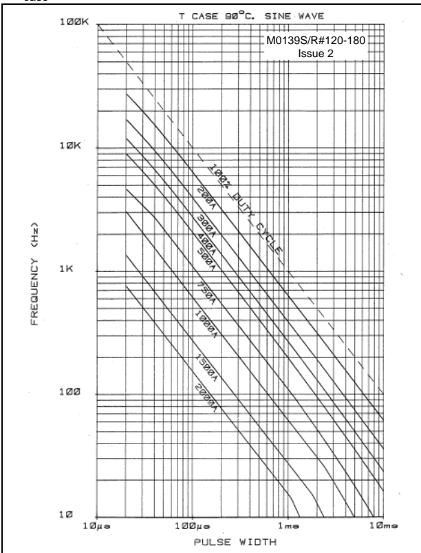
Figure 6 - Sine wave frequency vs. pulse width, T case - 90°C
