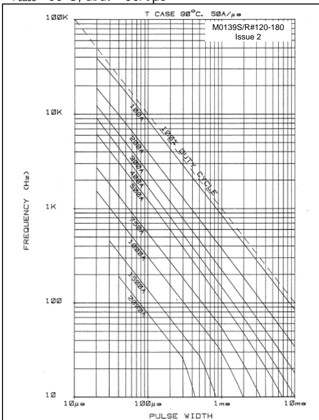
Figure 10 - Square wave frequency vs. pulse width, T_{\text{case}} - 90^\circ\text{C} , di/dt - 50\text{A}/\mu\text{s}
