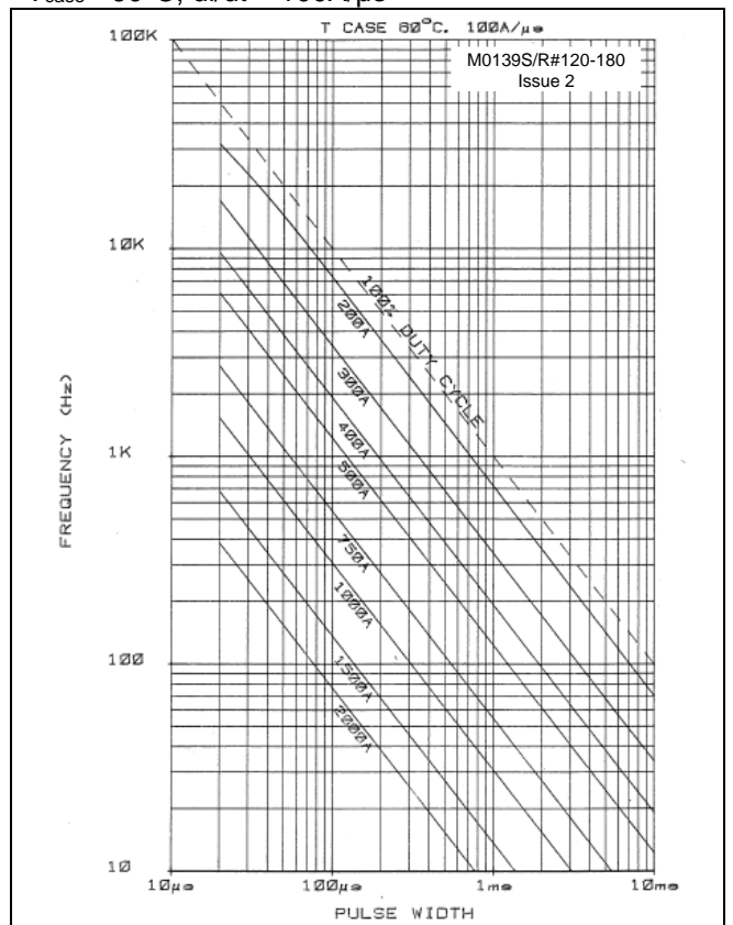
Figure 11 - Square wave frequency vs. pulse width, T_{\text{case}} - 60^\circ\text{C} , di/dt - 100\text{A}/\mu\text{s}
