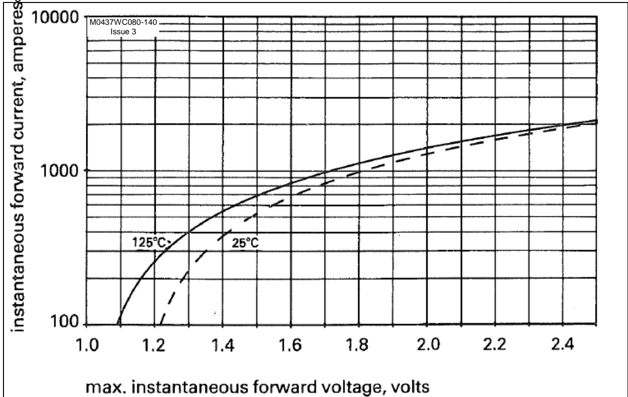
Figure 1 – Forward characteristics of Limit device
