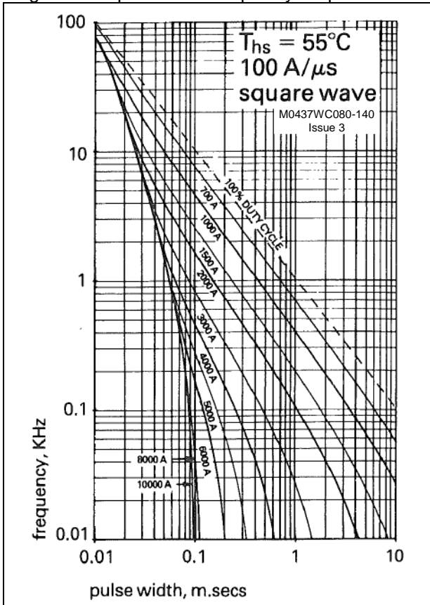
Figure 4 - Square wave frequency vs. pulse width
