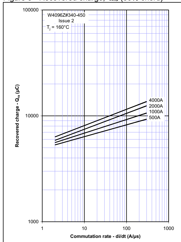
Figure 5 - Recovered charge, Q_{ra} (50% chord) ( \mu\text{C} )
