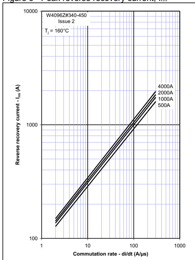
Figure 6 - Peak reverse recovery current, I_{rm} (A)
