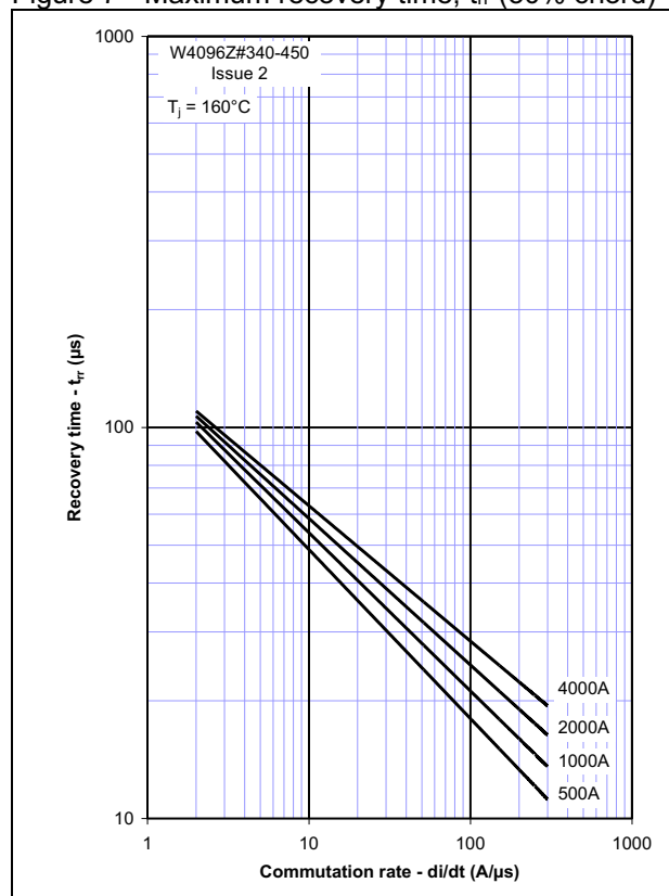
Figure 7 - Maximum recovery time, t_{rr} (50% chord) ( \mu\text{s} )
