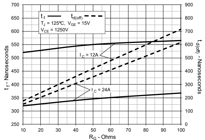
Fig. 20. Resistive Turn-off Switching Times vs. Gate Resistance
