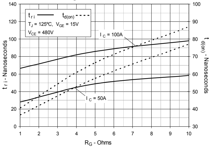
Fig. 17. Inductive Turn-on Switching Times vs. Gate Resistance
